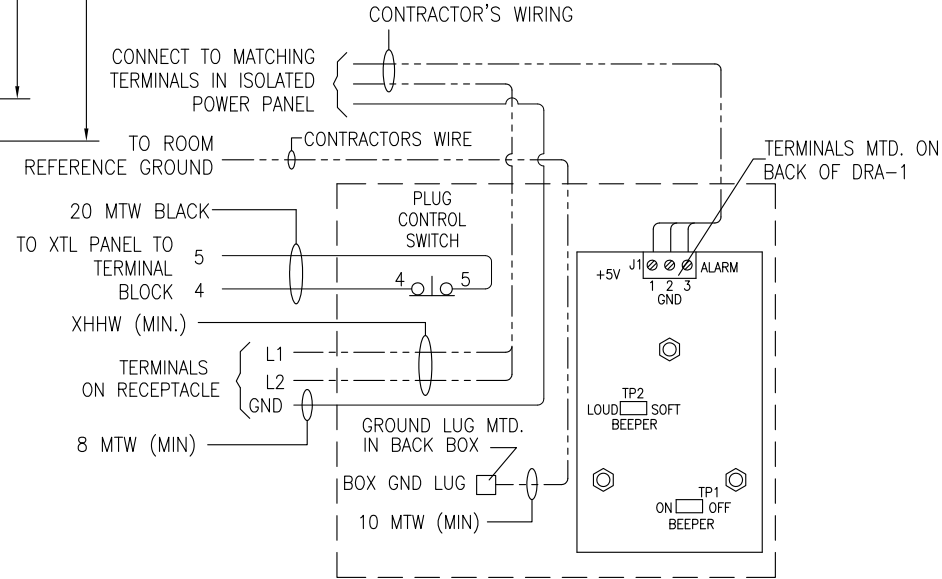
WIRING DIAGRAM
