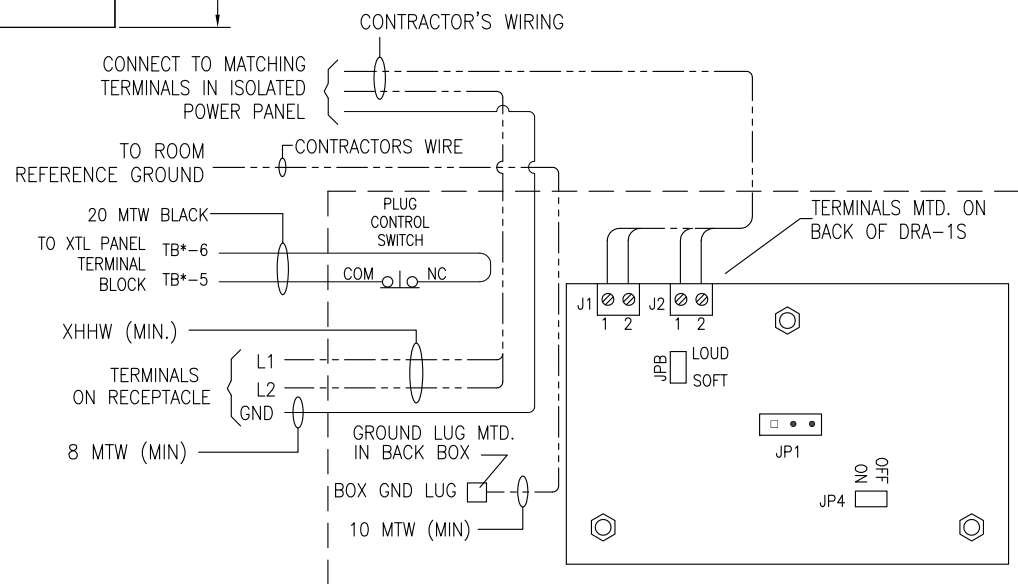
WIRING DIAGRAM
