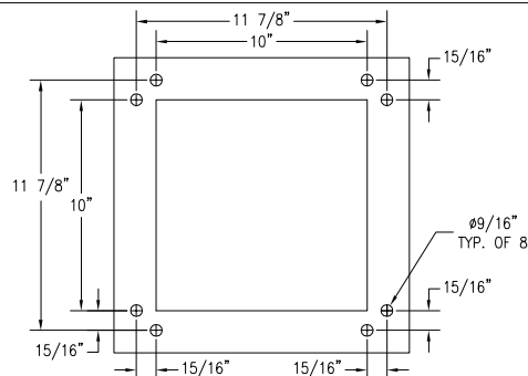
MOUNTING DETAIL
