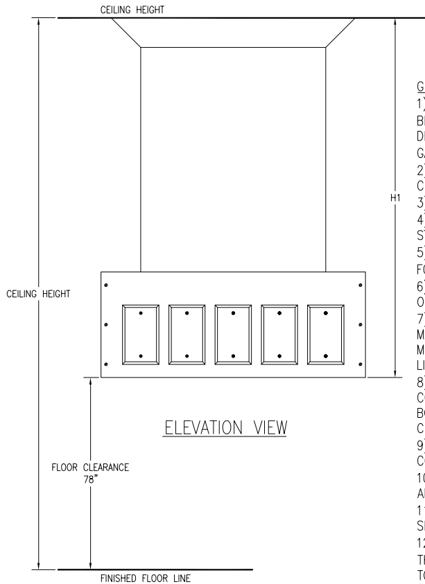
MOUNTING DETAIL
